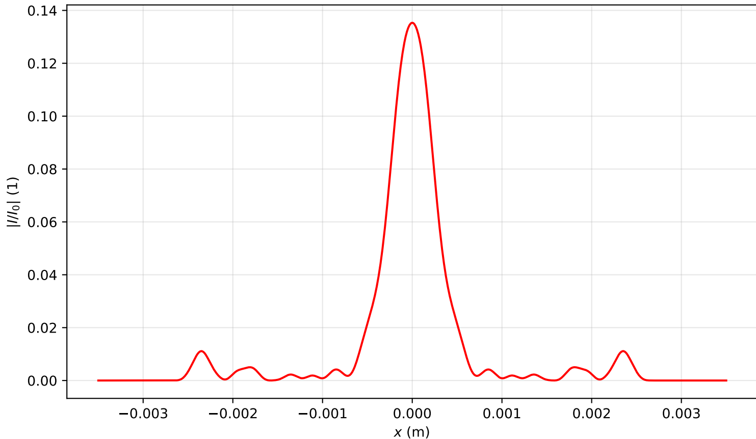
Intensity profile I(x, y = 0, z = 3.184)/I_0 , P_{in}=9.0P_{cr} , artificial time
